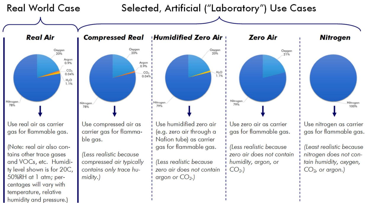
Figure 20: Various "air" options for use as the carrier, or background, gas during flammable gas testing. The best practice is to use one of the options toward the left side of the figure. In addition, do not switch between two different types of "air" during an experiment, as this can produce unwanted (and unrealistic) testing artifacts.
