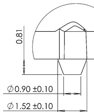
Figure 17: MPS Mini package pin dimensions, in mm.
