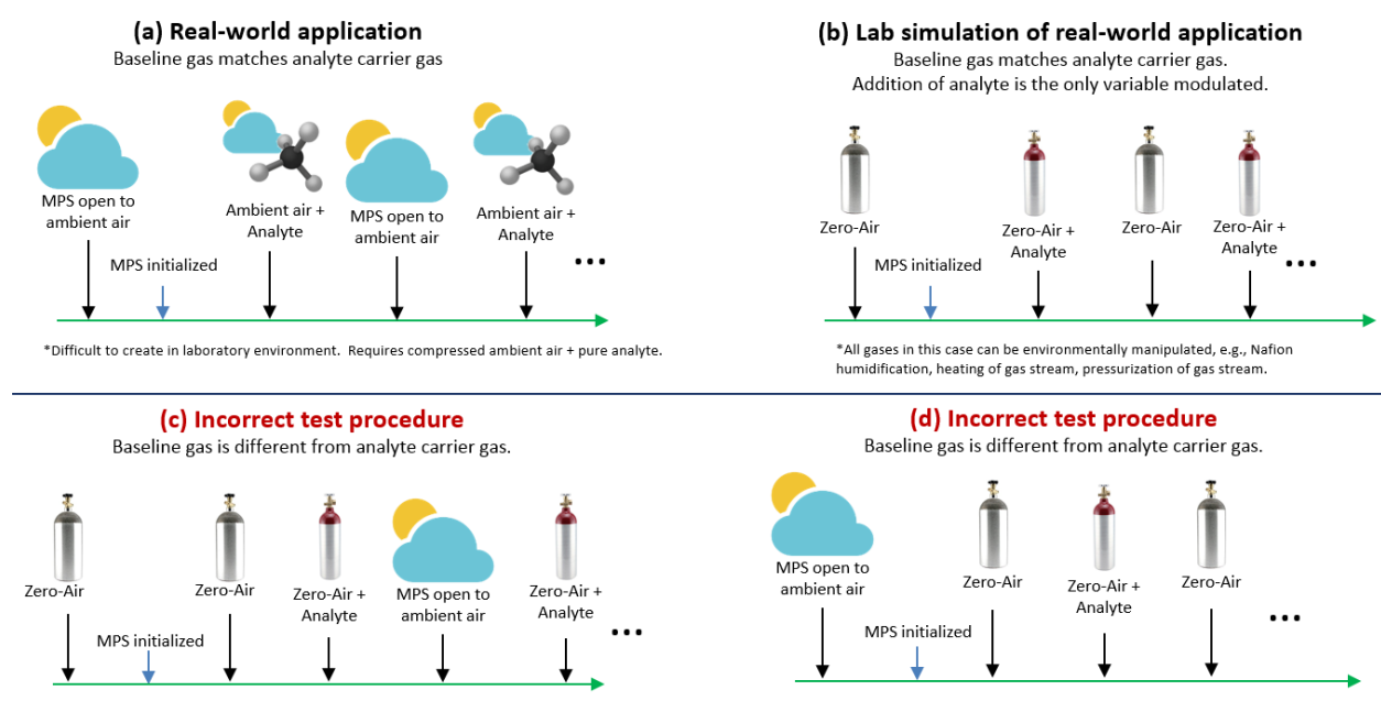
Figure 10: a) The real-world flammable gas leak scenario. (b) The method for simulating the real-world scenario in a laboratory. Incorrect test procedures are shown in (c) and (d); in these cases, the carrier-only condition does not use the same “air” as the carrier + flammable gas condition, causing inaccurate results.
