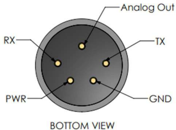
Figure 7: A2L IS electrical pin configuration
