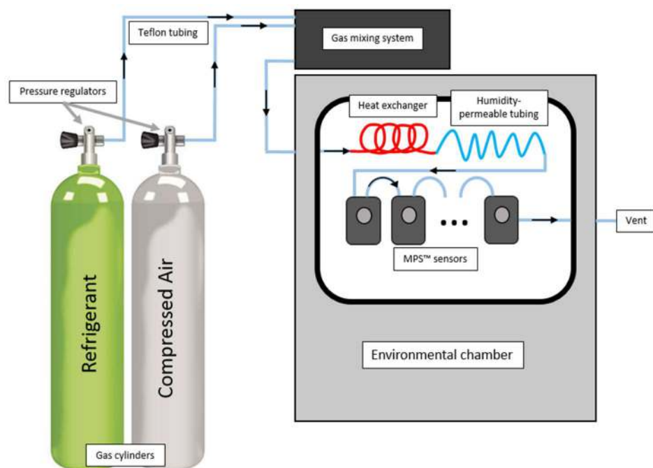
Figure 11: Setup #2: Testing in Various Environmental Conditions
