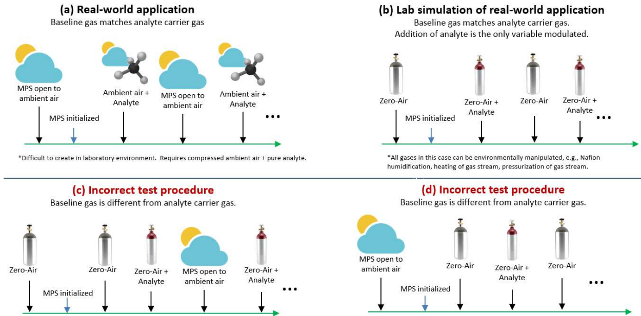
Figure 12: (a) The real-world flammable gas leak scenario. (b) The method for simulating the real-world scenario in a laboratory. Incorrect test procedures are shown in (c) and (d); in these cases, the carrier-only condition does not use the same “air” as the carrier + flammable gas condition, causing inaccurate results.
