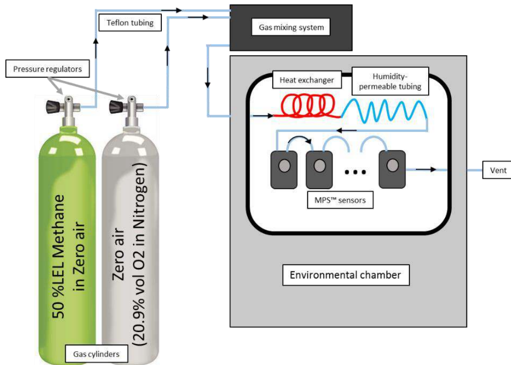
Figure 14: Setup #1: Gas Testing in Various Environmental Conditions
