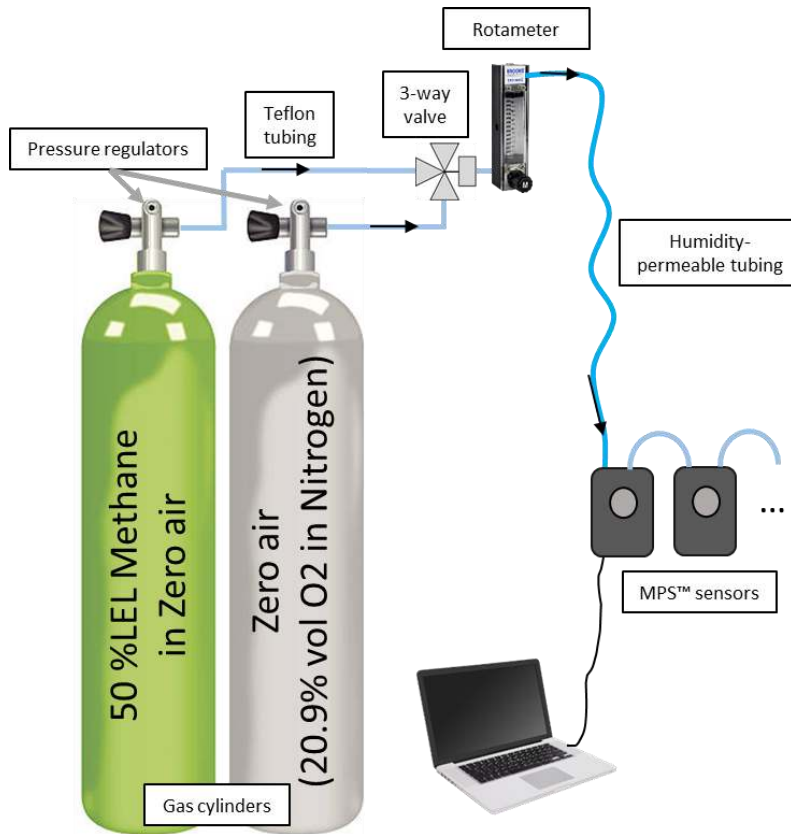
Figure 15: Setup #2: General benchtop testing.
