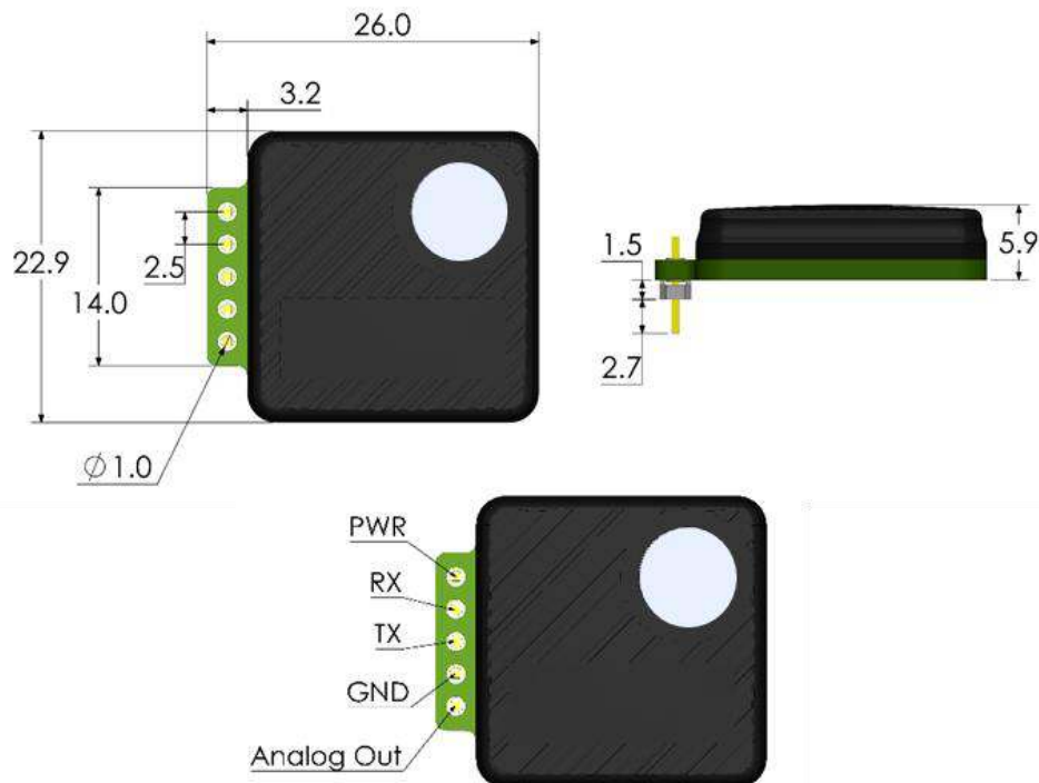
Figure 11: MPS Flammable Gas Sensor Mini form factor mechanical dimensions (in mm) and pinout.
