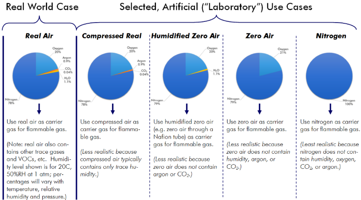
Figure 13: Various “air” options for use as the carrier, or background, gas during flammable gas testing. The best practice is to use one of the options toward the left side of the figure. In addition, do not switch between two different types of “air” during an experiment, as this can produce unwanted (and unrealistic) testing artifacts.
