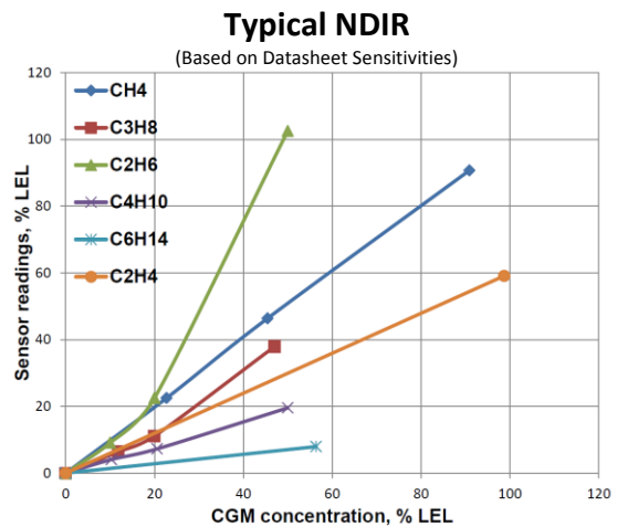
Figure 1: The delivered vs. reported concentrations of selected flammable gases, for each of the three sensor types when calibrated to methane.
